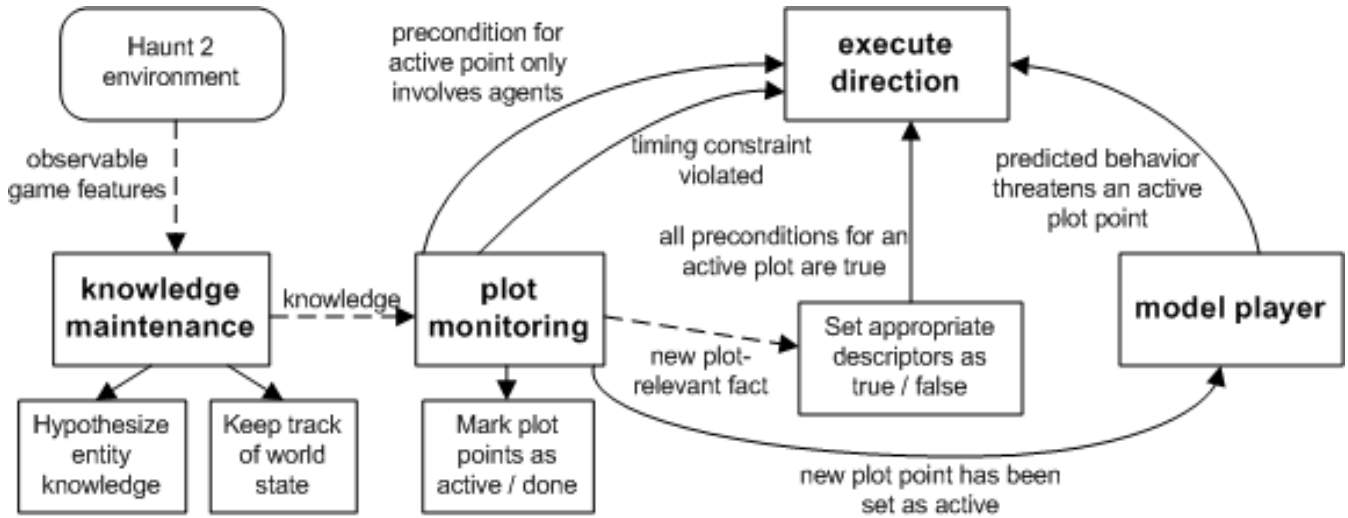
Figure 1. The execution cycle of the director agent.
